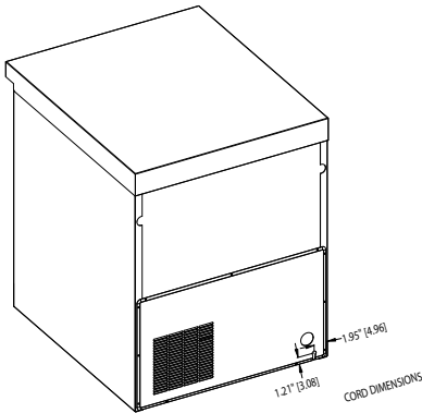
UC4427N & UCD4427N REAR ISO VIEW
