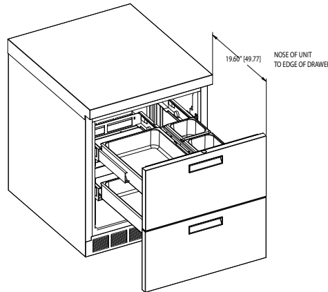
UCD4427N ISO VIEW
