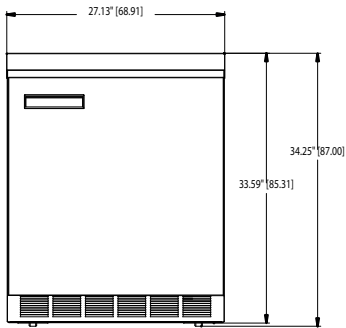
UC4427N ELEVATION VIEW
