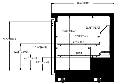
UC4427N RIGHT SIDE VIEW
