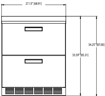
UCD4427N ELEVATION VIEW
