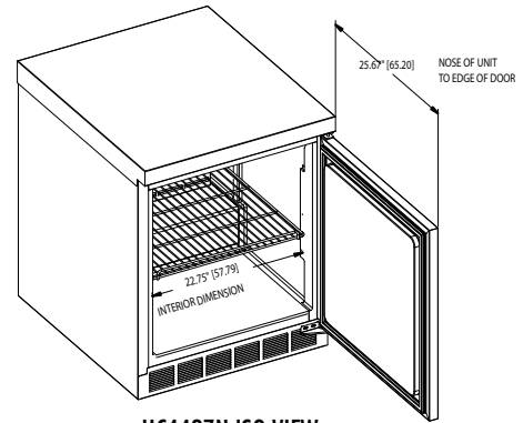
UC4427N ISO VIEW
