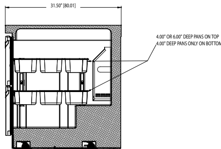
UCD4427N RIGHT SIDE VIEW
